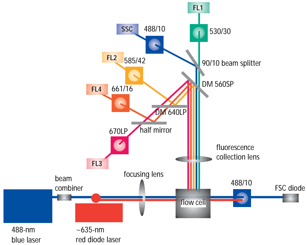
Figure 1-7 Optics system with FL4 option
